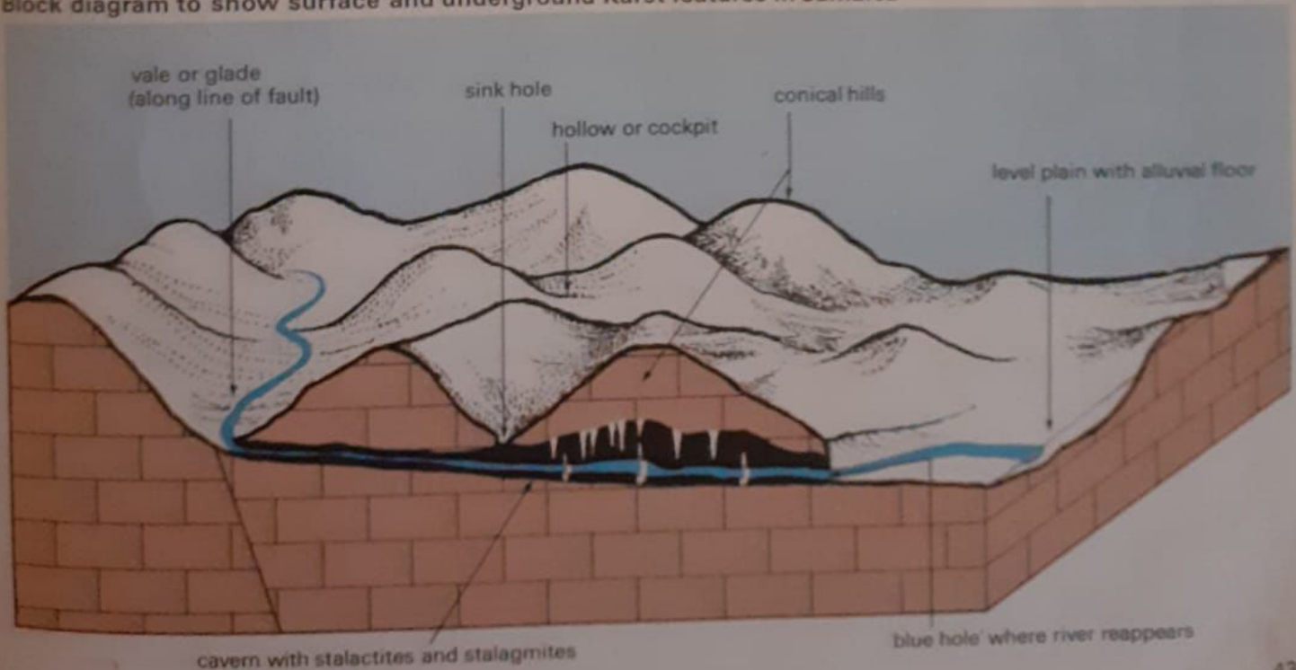
Block diagram to show surface and underground Karst features in Jamaica
